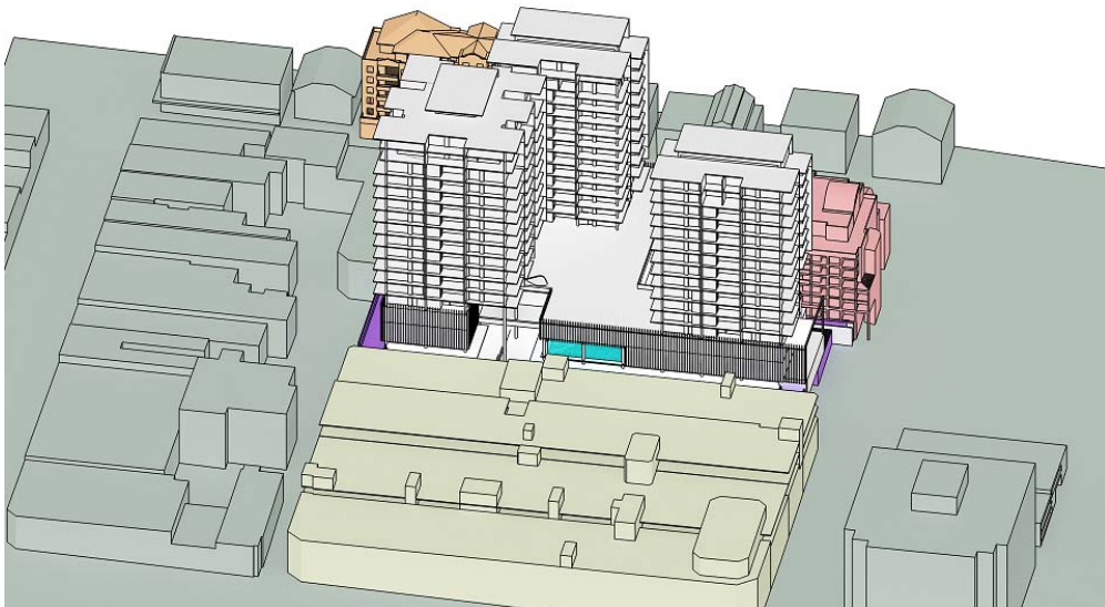
Figure 4: Solar Access 12 noon winter (final scheme)
